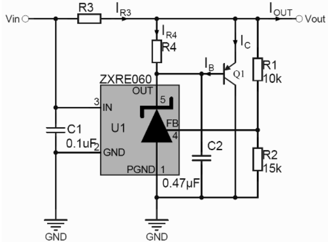
Figure 6. 1V Current-boosted Shunt Regulator
