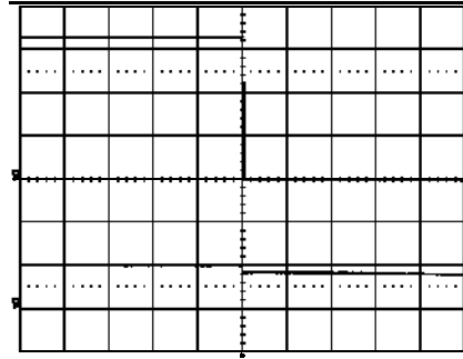
Shut-down enabled by disconnecting V_i at: T_{ref} = +25^{\circ}\text{C} , I_O = 6\text{ A} resistive load, V_i = 3.3\text{ V} . Top trace: output voltage (1.0 V/div.). Bottom trace: input voltage (5 V/div.). Time scale: 20.0 ms/div..
