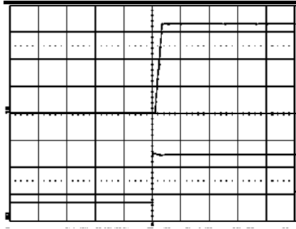
Start-up enabled by connecting V_i at: T_{ref} = +25^{\circ}\text{C} , I_O = 6\text{ A} resistive load, V_i = 5.0\text{ V} . Top trace: output voltage (1.0 V/div.). Bottom trace: input voltage (2 V/div.). Time scale: 20 ms/div..
