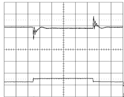
Output voltage response to load current step- change (3-6-3 A) at: T_{ref} = +25^{\circ}\text{C} , V_i = 5.0\text{ V} . Top trace: output voltage (100mV/div.). Bottom trace: load current (10 A/div.). Time scale: 0.1 ms/div.
