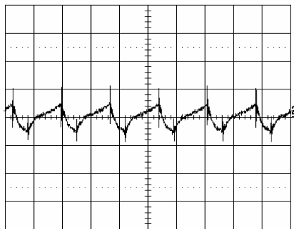
Output voltage ripple (20mV/div.) at: T_{ref} = +25^{\circ}\text{C} , I_O = 6\text{ A} resistive load, V_i = 5.0\text{ V} . Time scale: 1 \mu\text{s}/\text{div} . See the filter in the Output ripple and noise section (EMC Specification).
