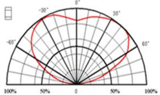
Directive Characteristics
