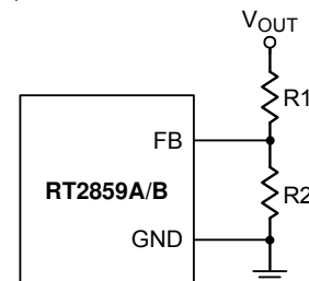
Figure 4. Output Voltage Setting
