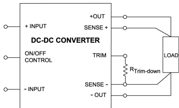
Fig. 3: Circuit configuration for Trim-down function
