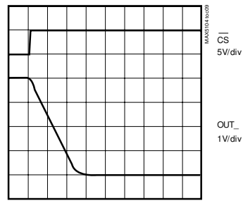
DYNAMIC RESPONSE FALL TIME
