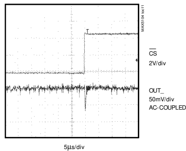
MAJOR-CARRY TRANSITION
