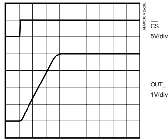
DYNAMIC RESPONSE RISE TIME
