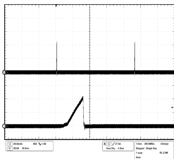
Fig.12: Load current (top trace, 20A/div, 50ms/div) into a 10m \Omega short circuit during restart, at V_{in} = 48V . Bottom trace (20A/div, 1ms/div) is an expansion of the top trace.
