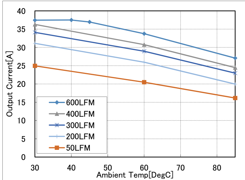
Fig.1-a: Available load current vs. ambient temperature and airflow rates for V_{in}=48V with baseplate. Airflow is from Pin 3 to Pin 1. Maximum component temperature \leq 125^{\circ}C
