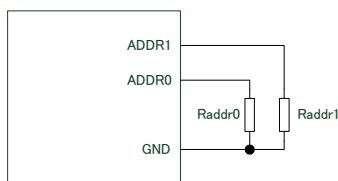
Fig. H. Circuit showing connection of resistors used to set the PMBus address of the module.
