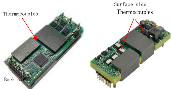
Fig. G: Location of thermocouples for thermal testing
