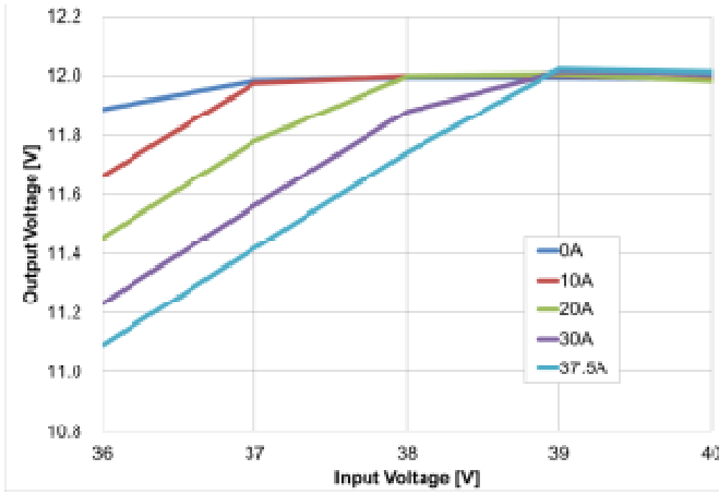
Fig.13: Vout vs. Vin at output voltage setting = 12 V. Power supply module 600 LFM (3.0 m / s) and Ta = 25 ° C horizontally mounted
