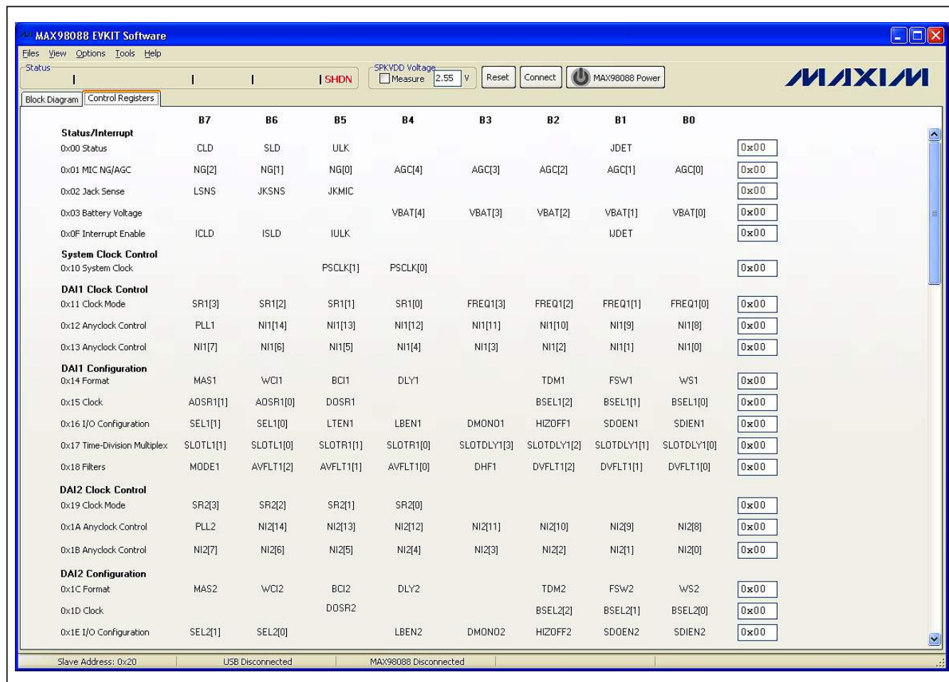
Figure 3. MAX98088 EV Kit Software Main Window (Control Registers Tab)
