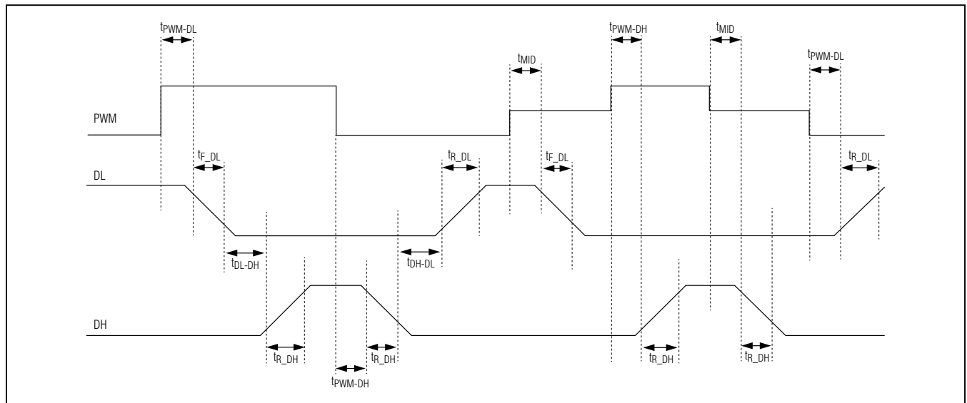
Figure 2. Timing Diagram
