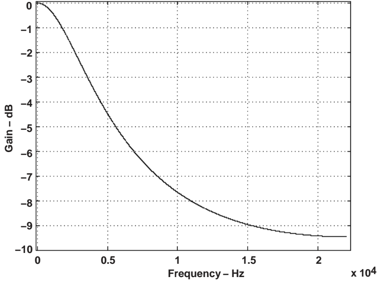
Digital De-Emphasis Frequency Response For F_s = 44.1 \text{ kHz}
