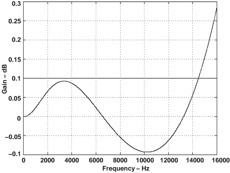
De-Emphasis Error With Respect to Ideal Frequency Response For F_s = 33 \text{ kHz}
