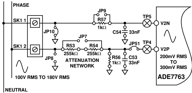
Figure 6. Voltage Channel on the ADE7763 Evaluation Board
