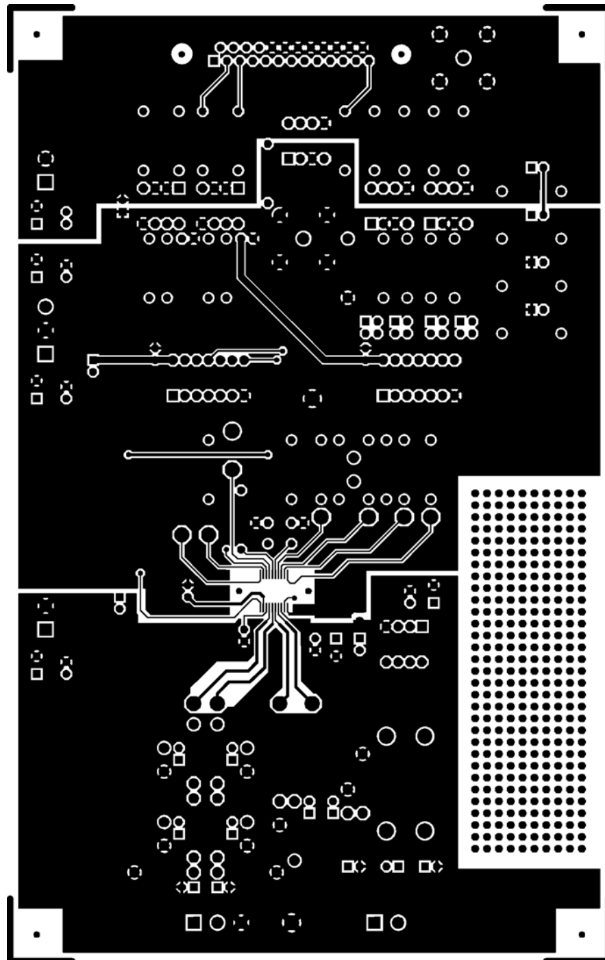
Figure 18. PCB Layout—Component Side
