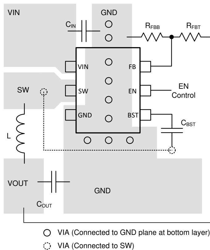
Figure 11-1. TPS563207S Layout
