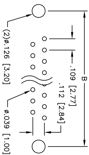
PCB LAYOUT
