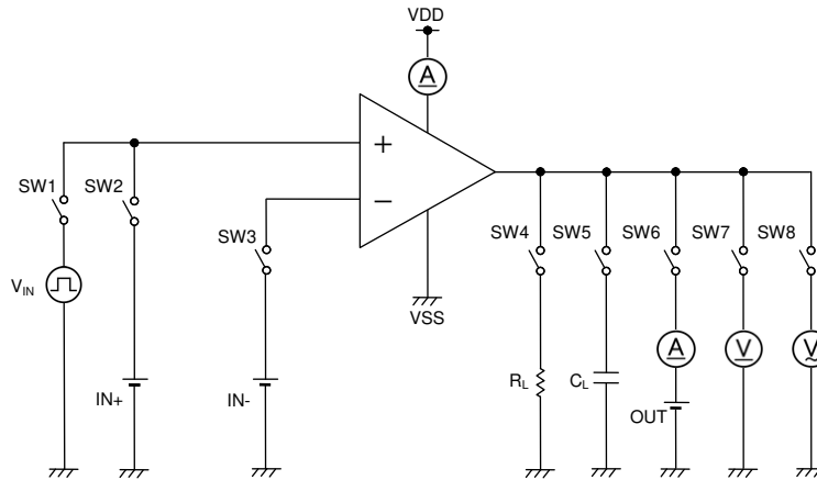
Figure 24. Test Circuit 2
