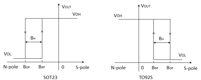
Magnetic Flux
