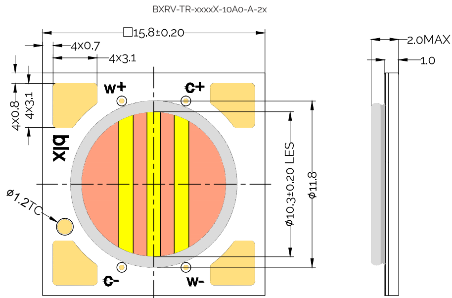
Figure 38: Drawing for Vesta Series Tunable White Gen2 9mm, 18V Array
