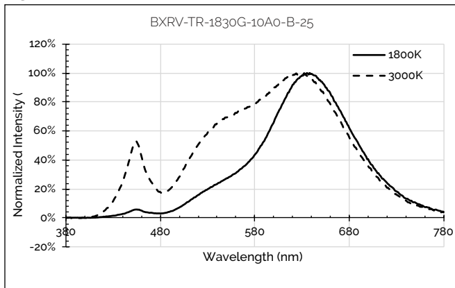
Figure 35: 1800K - 3000K with 90 CRI
