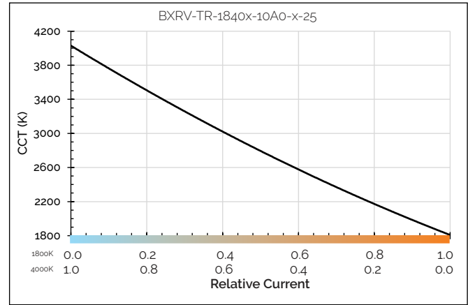
Figure 21: CCT vs. Relative Current, Tc=85C
