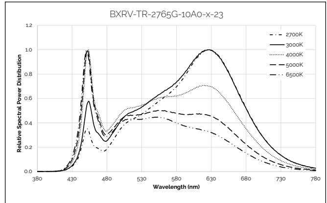
Figure 34: 2700K - 6500K with 90 CRI
