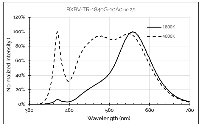
Figure 36: 1800K - 4000K with 90 CRI
