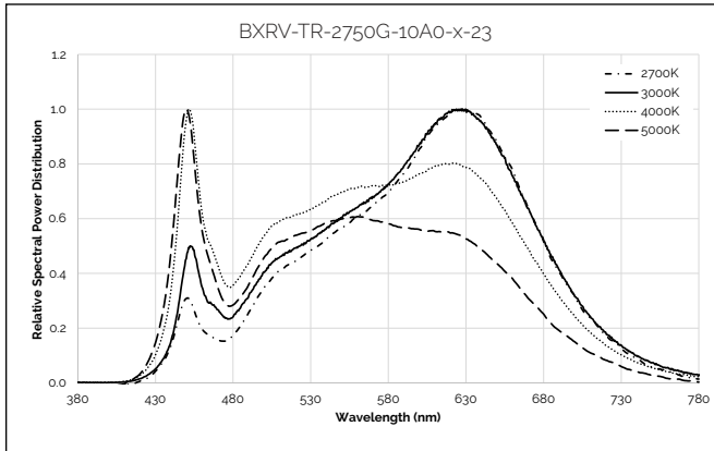
Figure 33: 2700K - 5000K with 90 CRI
