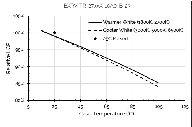
Figure 13: Relative Flux vs. Case Temperature
