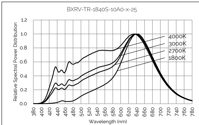
Figure 32: 1800K - 4000K with Thrive
