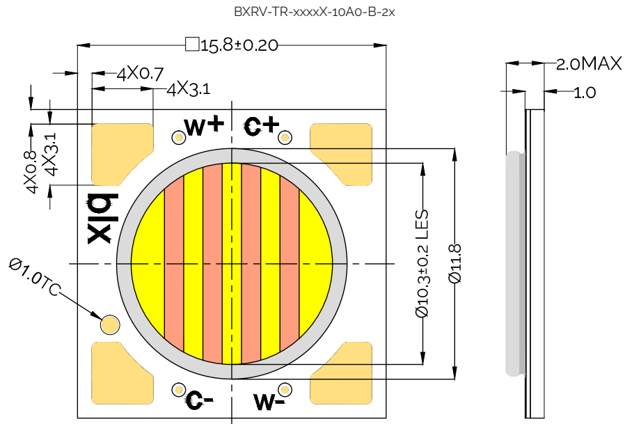
Figure 37: Drawing for Vesta Series Tunable White Gen2 9mm, 36V Array
