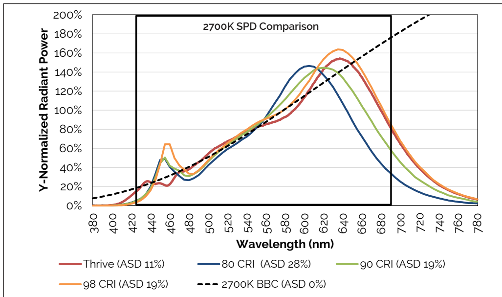
Figure 5: SPD Comparison
