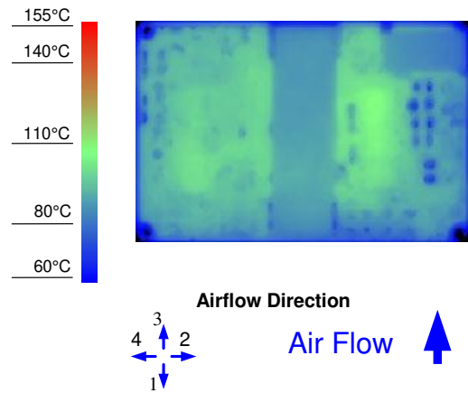
Figure 8. Thermal Image for Airflow Direction 3 (30.5A output, 55°C ambient, 200 LFM, typical Vin, open frame, unit soldered onto a fixture board)
