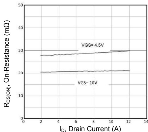
Figure 4. On-Resistance vs. Drain Current and V_{GS}
