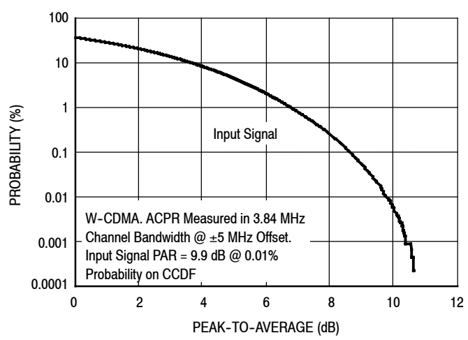
Figure 8. CCDF W-CDMA IQ Magnitude Clipping, Single-Carrier Test Signal
