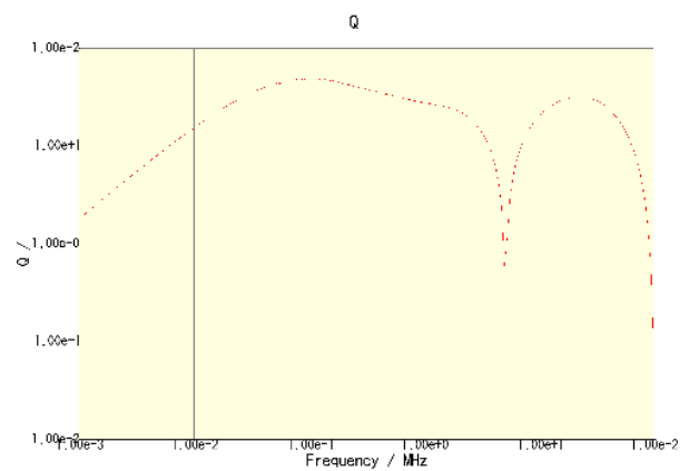
CLF6045T-101M-CA
