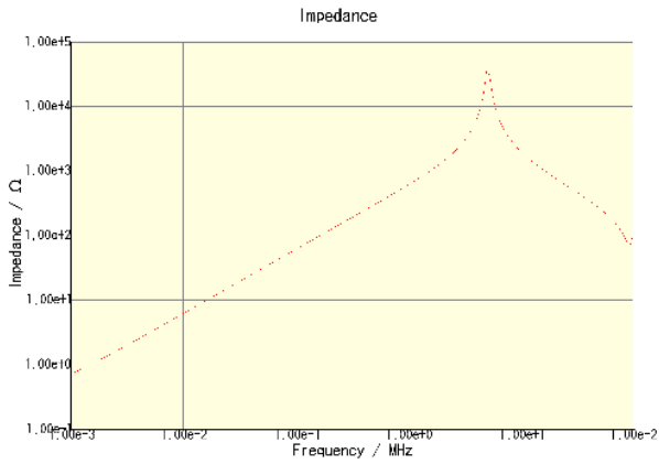
CLF6045T-101M-CA
