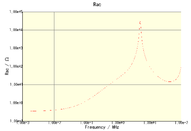
CLF6045T-101M-CA
