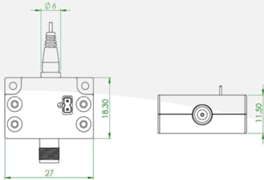
PD-30e-C Mechanical Drawing
