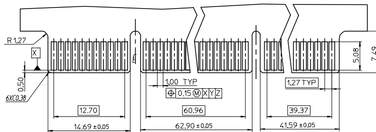
RECOMMENDED MATING P.CBOARD LAYOUT
