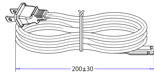
B-C2 扎線圖示 (Tied Loop Hank Detail)
