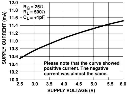
FIGURE 31. SUPPLY CURRENT vs SUPPLY VOLTAGE
