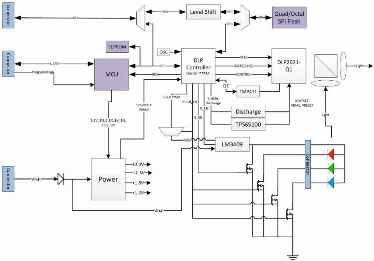
Figure 1-1. DLP2021LEQ1EVM Block Diagram
