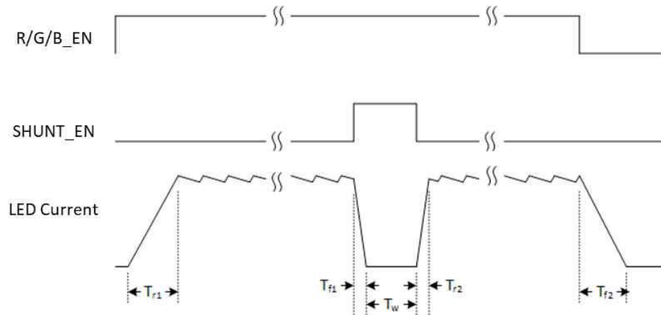
Figure 1-7. LED Driver Timing Specifications
