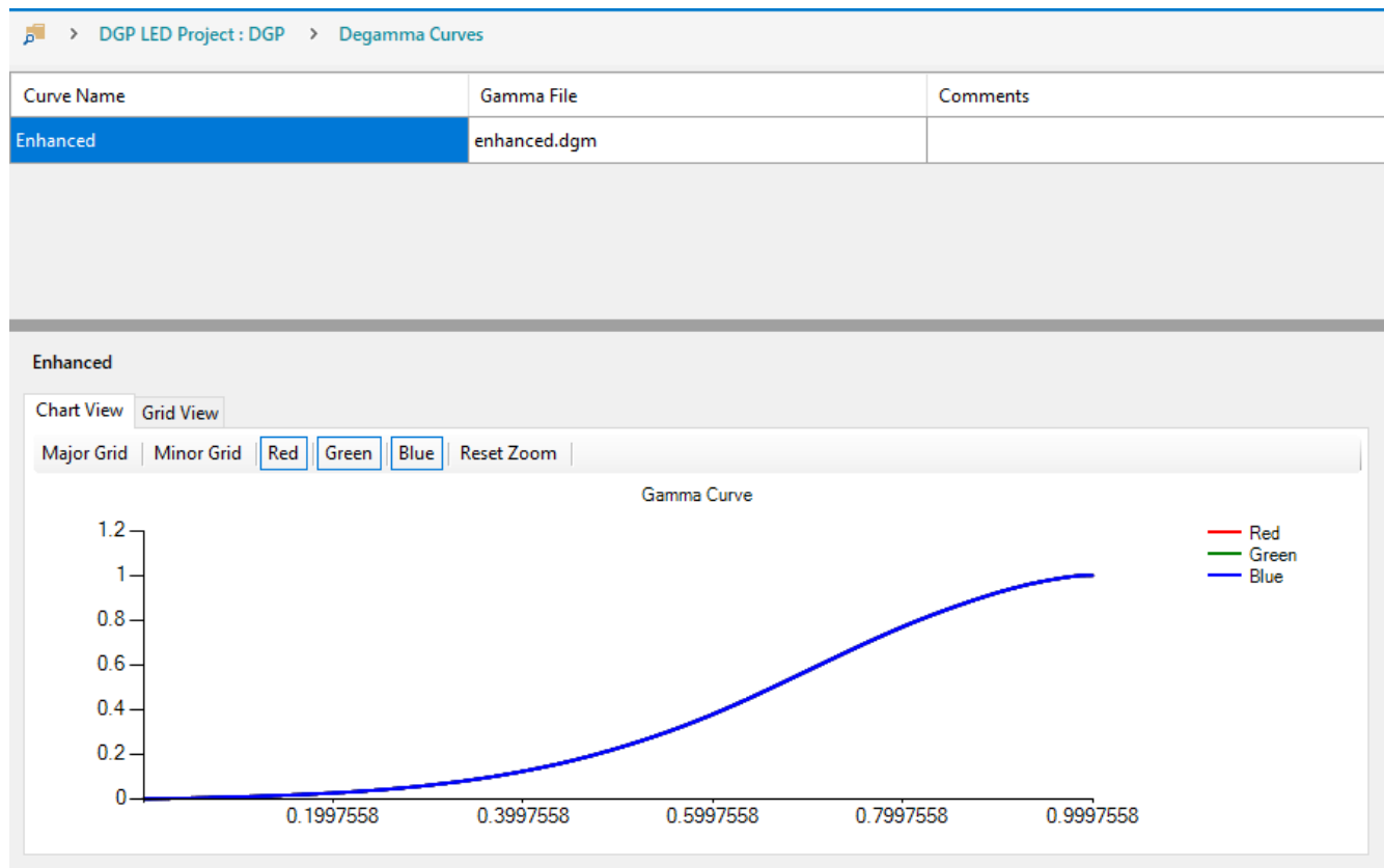
Figure 4-4. DLP Composer - Degamma Curves
