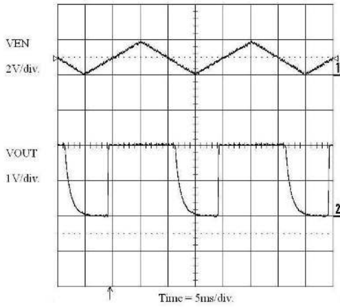
Figure 21. Slow Enable Operation (1 mA Load)
