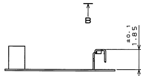
VIEW B (SCALE 2:1)
