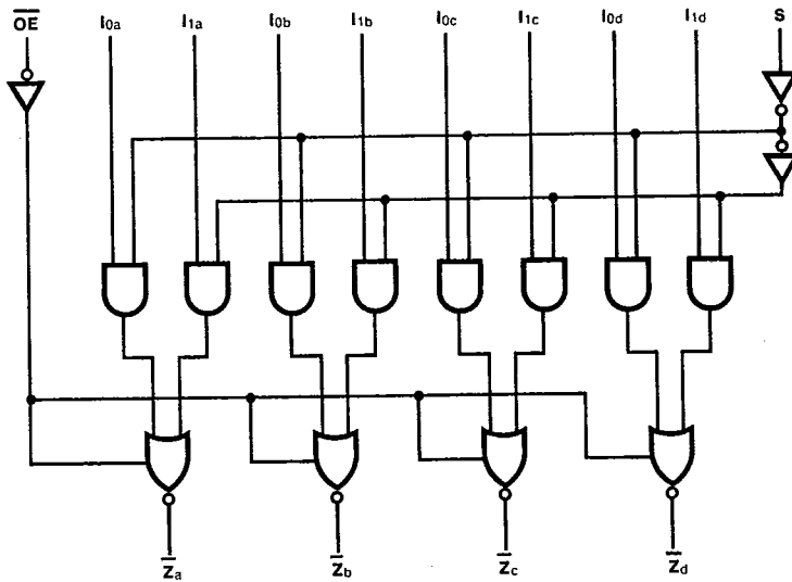
LOGIC DIAGRAM
