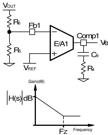
Figure 6 - Compensation network without local feedback and its asymptotic gain plot.
