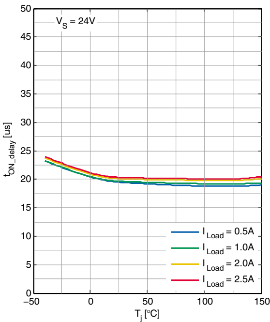
Turn-ON delay time t_{ON\_delay} to V_{OUT} = 10\% versus Junction Temperature T_j
