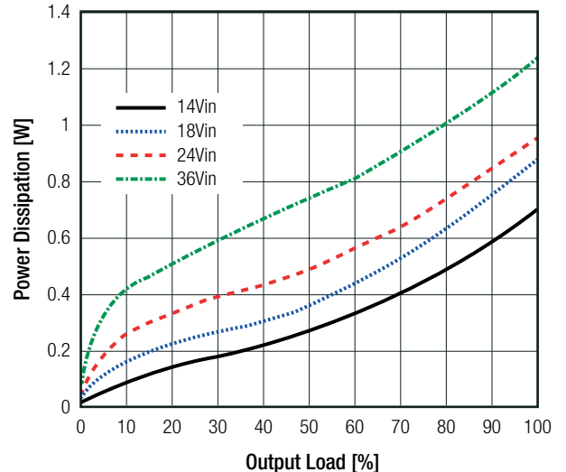
Power Dissipation vs. Load
