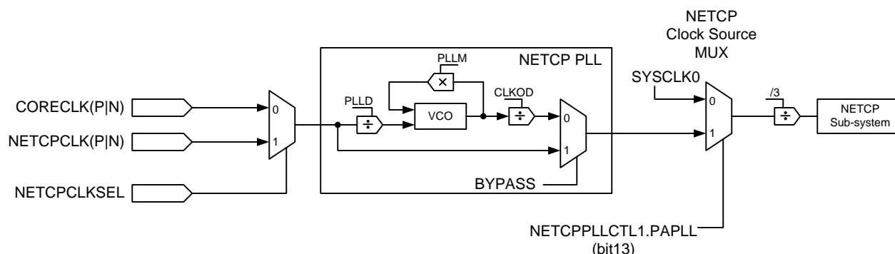
Figure 11-26. NETCP PLL Block Diagram
