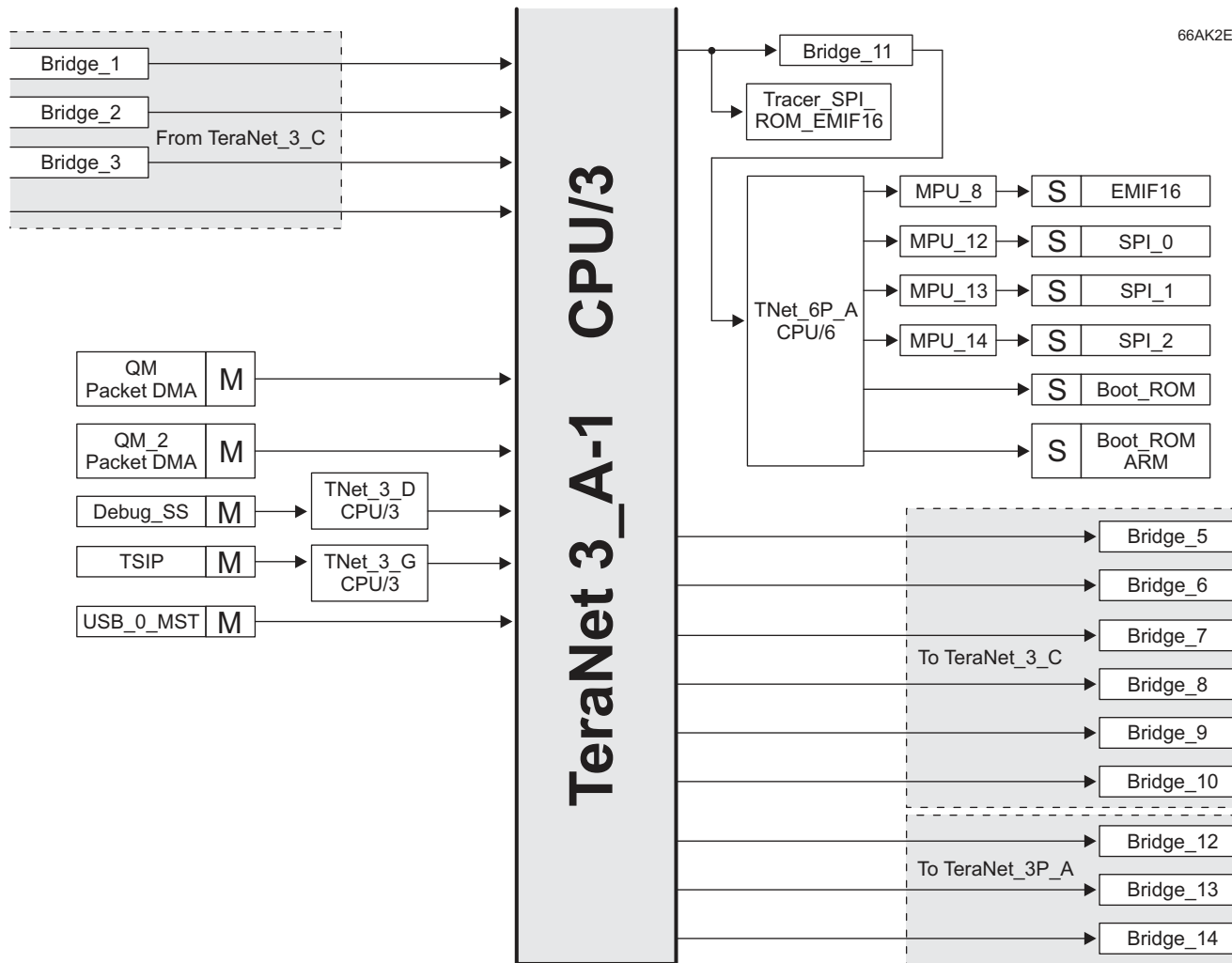
Figure 8-1. TeraNet 3_A-1
