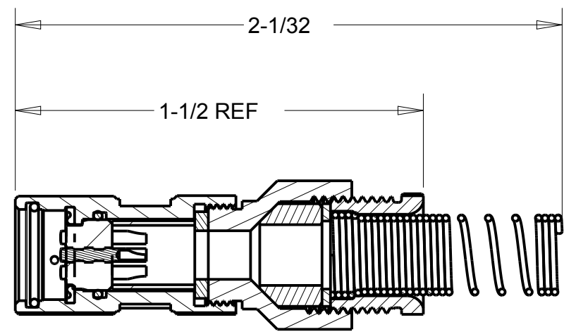
SECTION Z-Z
