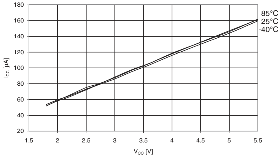
Figure 31-238. ATmega329PA: AREF external reference current vs. V_{CC} .
