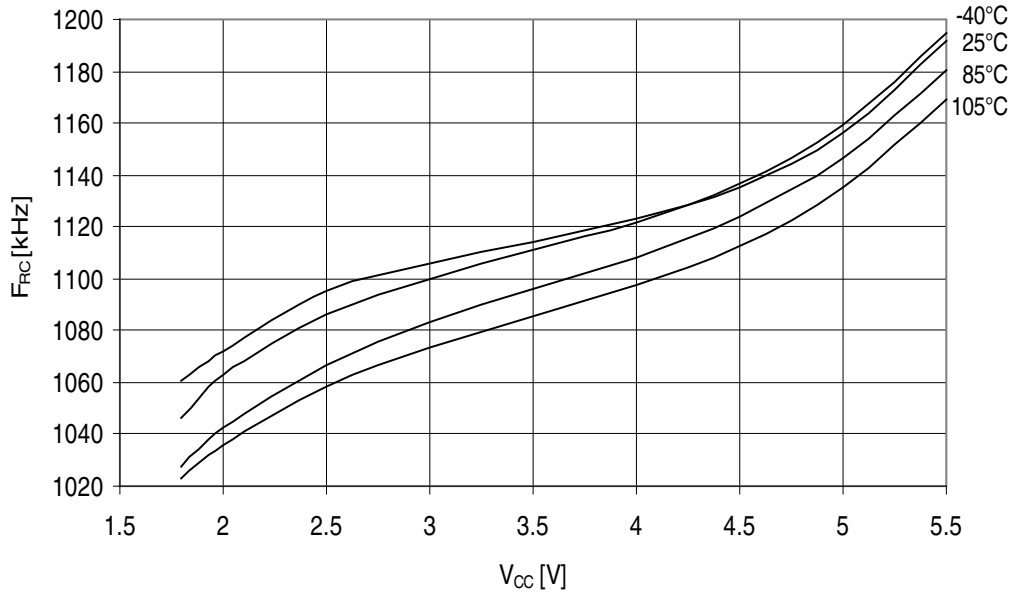
Figure 32-103. ATmega329A - 105°C: Watchdog Oscillator Frequency vs. V_{CC}
