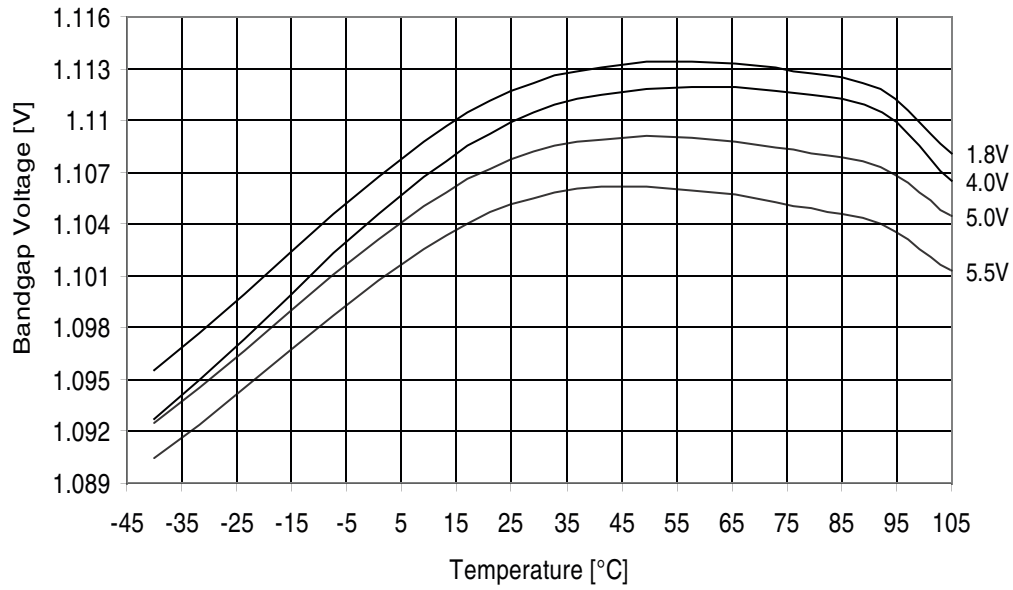
Figure 32-279. ATmega3290A: Bandgap Voltage vs. Temperature
