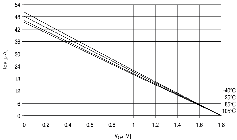
Figure 32-369. ATmega3290PA - 105°C: I/O Pin Pull-up Resistor Current vs. Input Voltage ( V_{CC} = 1.8V )
