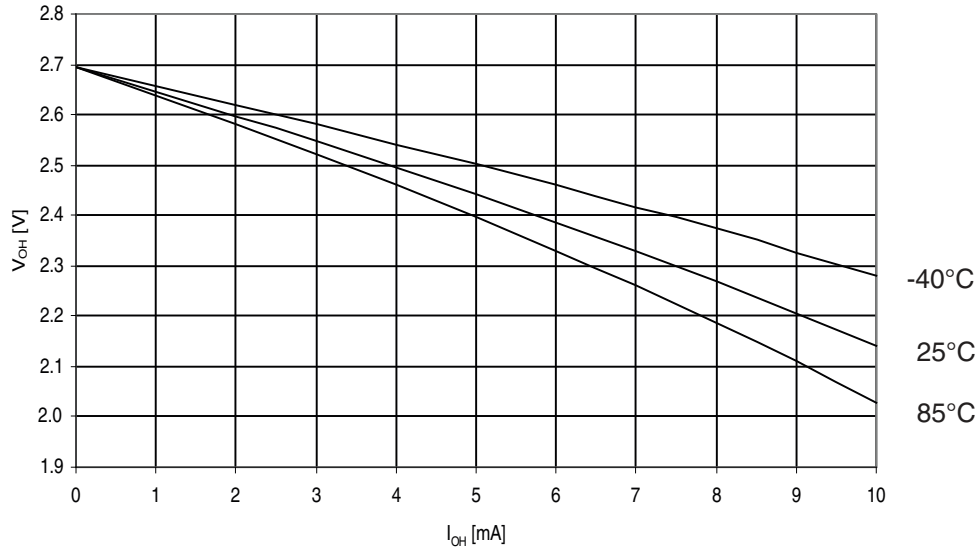
Figure 31-207. Atmel ATmega329PA: I/O pin output voltage vs. source current, ports A, C, D, E, F, G ( V_{CC} = 2.7V ).
