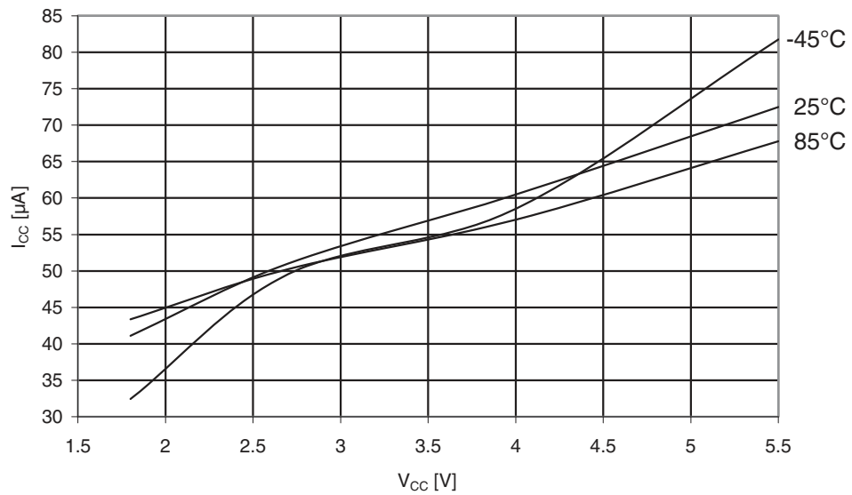
Figure 31-120. ATmega169PA: Analog Comparator current vs. V_{CC} .
