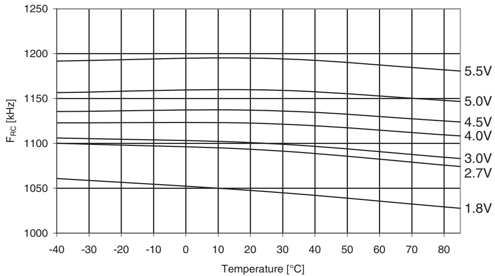
Figure 31-170. ATmega329A: Watchdog oscillator frequency vs. temperature.
