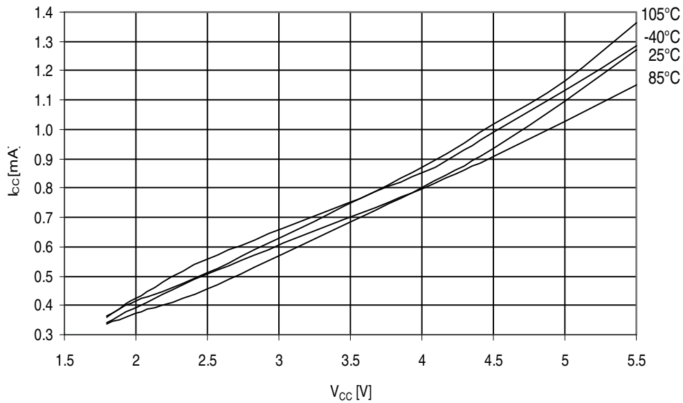
Figure 32-177. ATmega329PA - 105°C: Active Supply Current vs. V_{CC} (Internal RC Oscillator, 1MHz)
