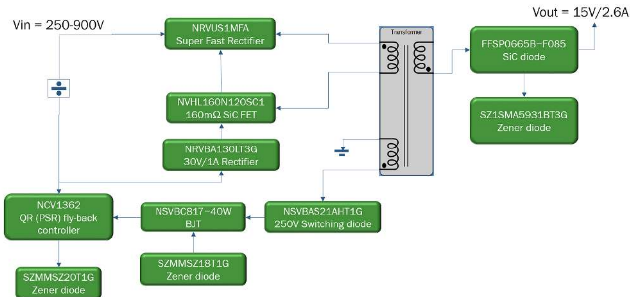
Figure 3. Block Diagram
