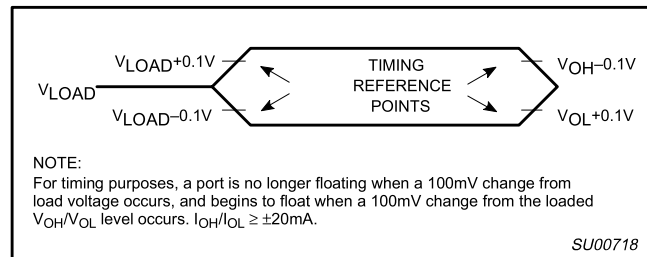
Figure 57. Float Waveform
