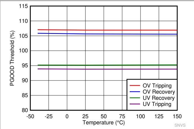
Figure 8-8. PGOOD Thresholds
