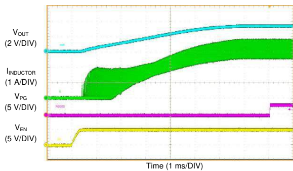
Figure 10-31. LMQ61460-Q1 Start-up with 50-mA Load
