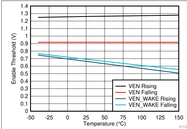
Figure 8-7. Enable Thresholds
