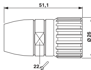
Dimensioned drawing
