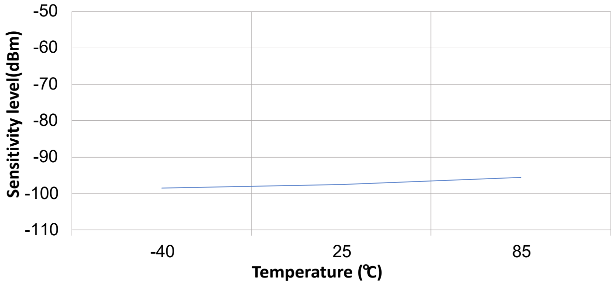
Figure 43-24. Module Bluetooth Low Energy Receive Sensitivity vs Temperature
