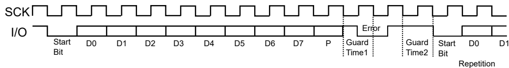
Figure 30-21. T=0 Protocol with Parity Error
