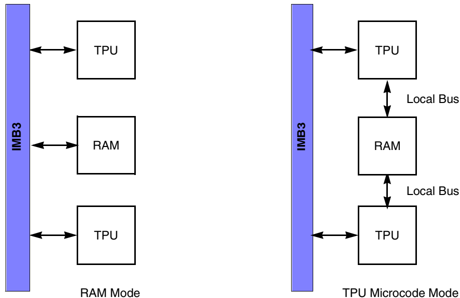
Figure 18-1 DPTRAM Configuration
