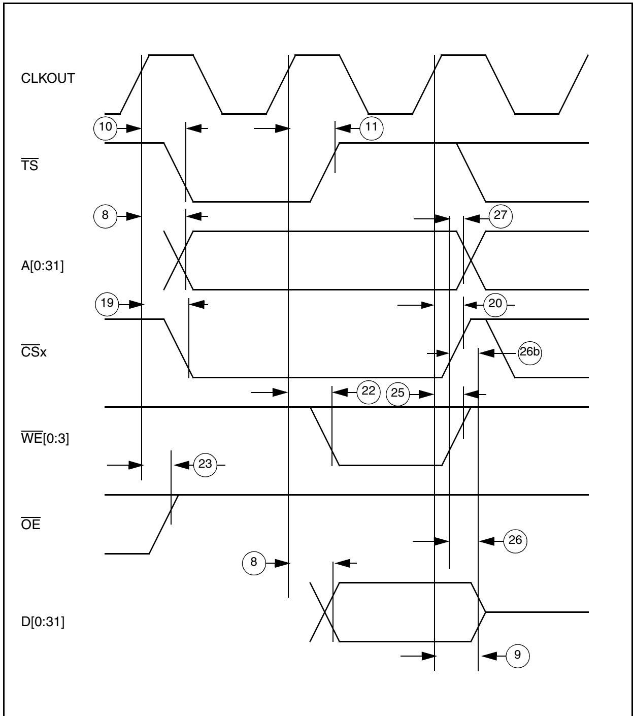
Figure G-13 External Bus Write Timing (GPCM Controlled — TRLX = '0', CSNT = '0')
