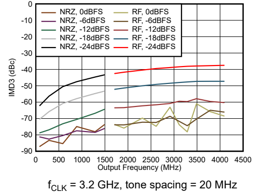
Figure 6-74. Dual Channel NRZ and RF Modes: IMD3 vs Output Frequency and Digital Level
