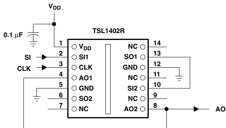
Figure 9. Serial Connection
