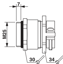
Dimensioned drawing
