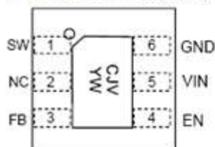
Top View U-DFN2020-6 (Type C)
