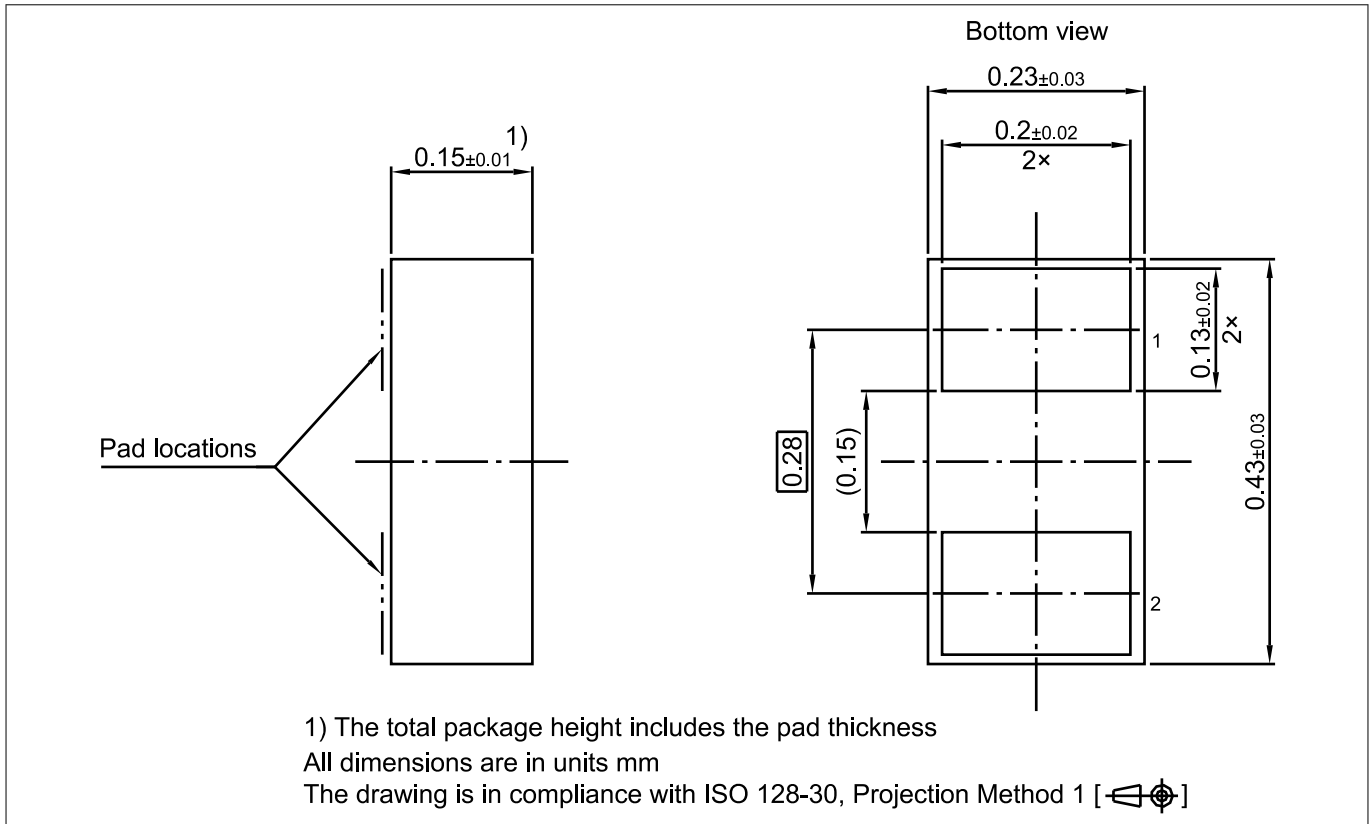
Figure 12 WLL-2-2 package
