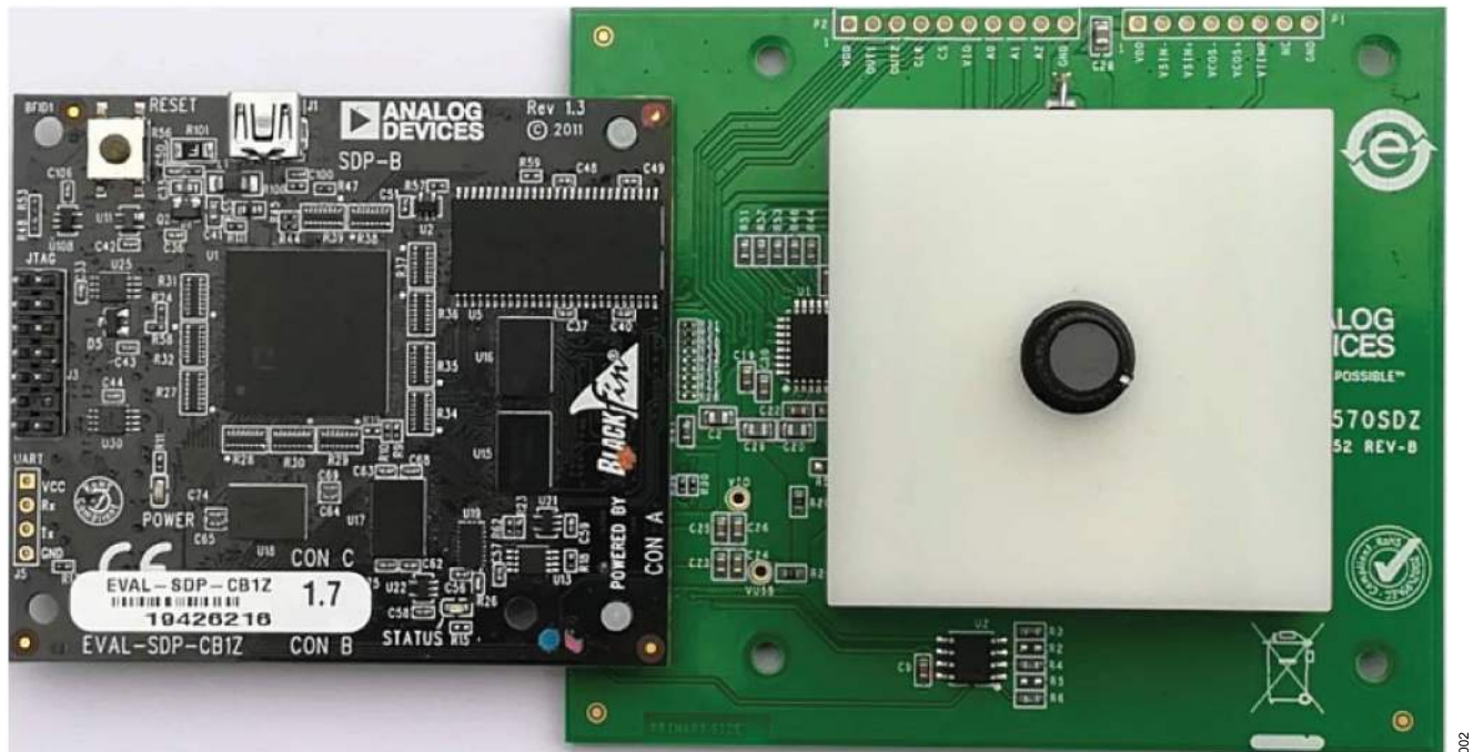
Figure 2. Hardware Configuration Showing the Demonstration Magnet Assembly, EVAL-ADA4570SDZ, and the SDP-B
