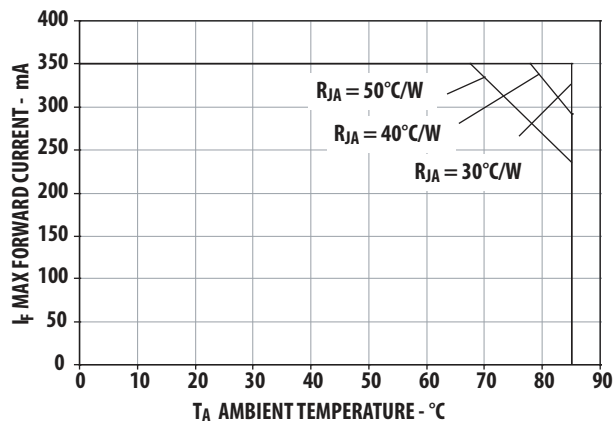
Figure 5. Maximum forward current vs. ambient temperature for AlInGaP Derated based on T_{jMAX} = 120^{\circ}C , R_{\theta JA} = 30^{\circ}C/W / 40^{\circ}C/W and 50^{\circ}C/W
