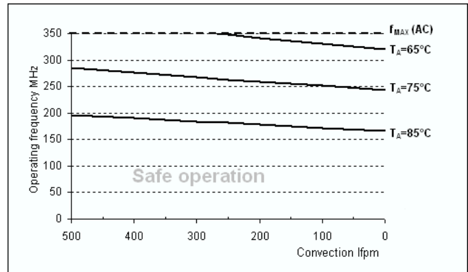
Figure 7. Maximum MPC9443 Frequency, V_{\text{CC}} = 3.3 \text{ V} , MTBF 9.1 Years, 4 pF Load per Line
