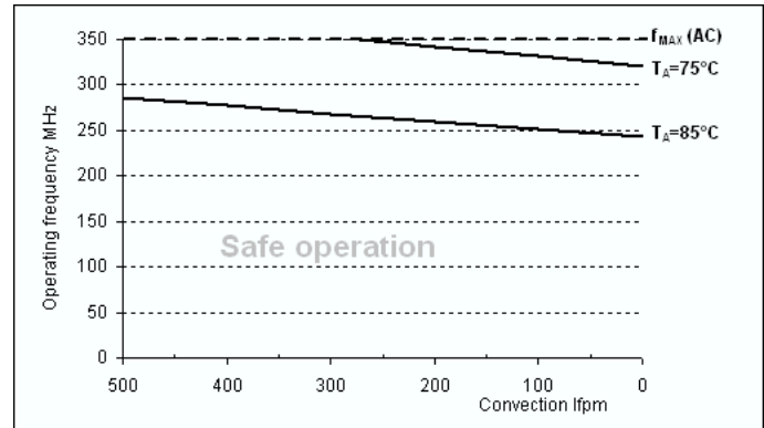
Figure 9. Maximum MPC9443 Frequency, V_{\text{CC}} = 3.3 \text{ V} , MTBF 4 Years, 4 pF Load per Line
