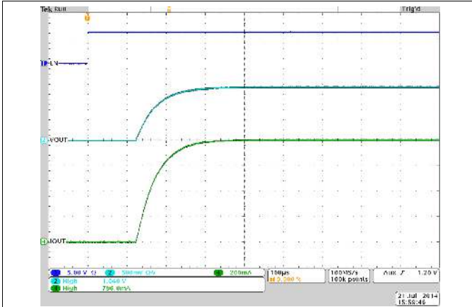
Figure 38. Startup for TPS8268105 (Vin = 5V, Vout = 1.05V)
