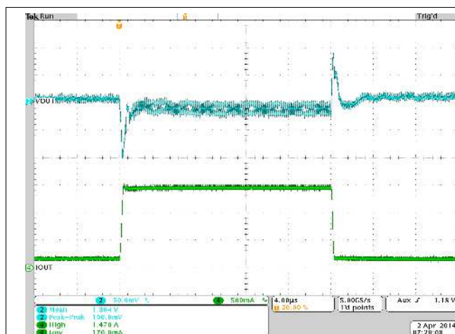
Figure 24. Load Transient Response for TPS8268180 ( V_{\text{out}} = 1.80\text{V} , I_{\text{out}} = 170\text{mA} to 1.47\text{A} to 170\text{mA} , V_{\text{in}} = 5\text{V} )
