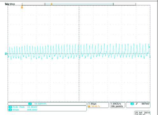
Figure 43. Output Voltage Ripple for TPS8268090 (Vin = 5V, Vout = 0.9V, Iout = 900mA)
