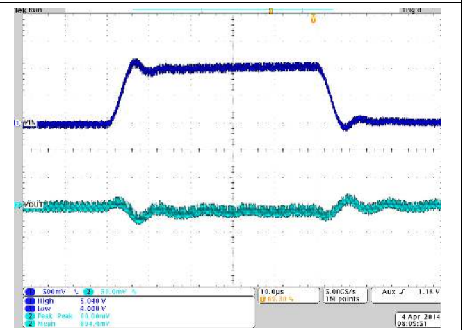
Figure 41. Line Transient Response for TPS8268090 (Vout = 0.90V; Iout = 900mA, Vin = 4V to 5V to 4V)
