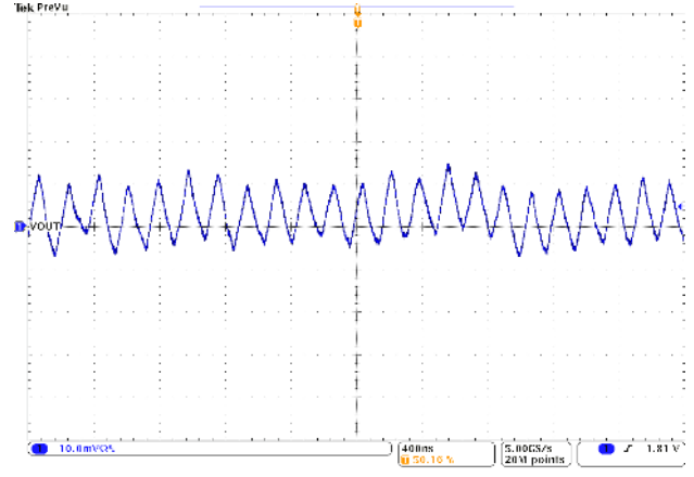
Figure 27. Output Voltage Ripple for TPS8268180 (Vin = 5V, Vout = 1.80V, Iout = 900mA)
