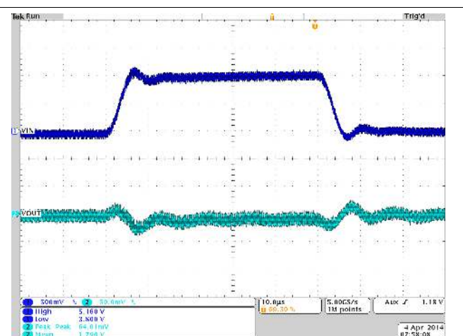
Figure 25. Line Transient Response for TPS8268180 ( V_{\text{out}} = 1.80\text{V} ; I_{\text{out}} = 800\text{mA} , V_{\text{in}} = 4\text{V} to 5\text{V} to 4\text{V} )
