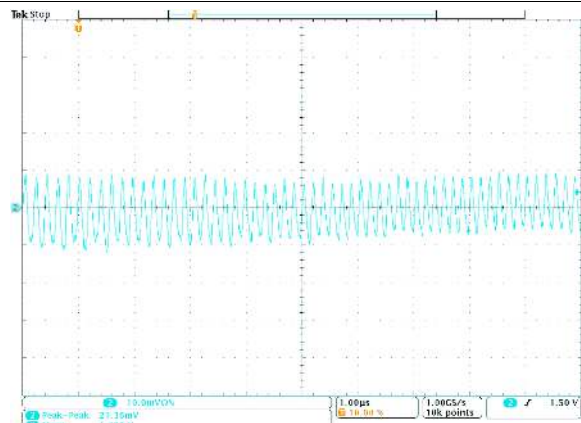
Figure 31. Output Voltage Ripple for TPS8268150 (Vin = 5V, Vout = 1.5V, Iout = 900mA)
