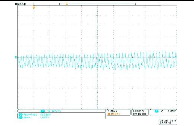
Figure 39. Output Voltage Ripple for TPS8268105 (Vin = 5V, Vout = 1.05V, Iout = 900mA)
