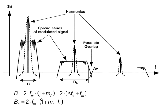
Figure 22. Spread Bands Of Harmonics In Modulated Square Signals (1)
