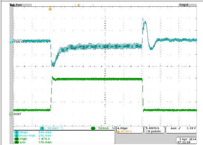
Figure 40. Load Transient Response for TPS8268090 (Vout = 0.9V, Iout = 170mA to 1.47A to 170mA, Vin = 5V)
