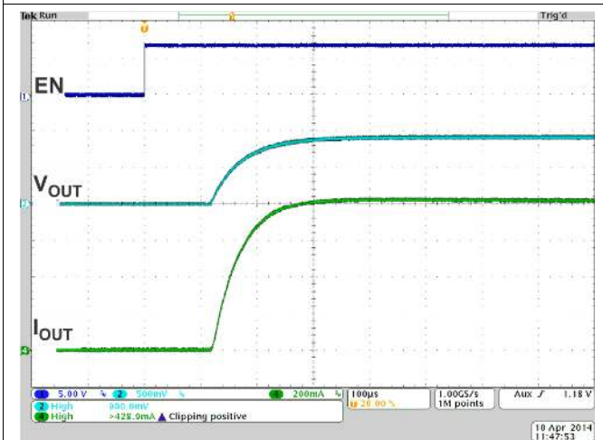
Figure 42. Startup for TPS8268090 (Vin = 5V, Vout = 0.9V)
