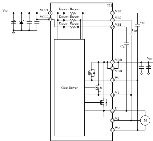
Figure 10-11. Bootstrap Circuit
