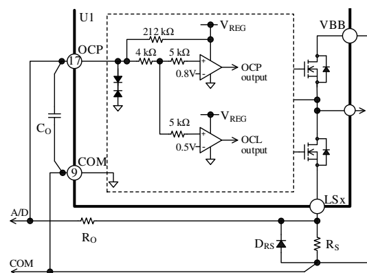
Figure 10-20. Internal Circuit Diagram of OCP Pin
