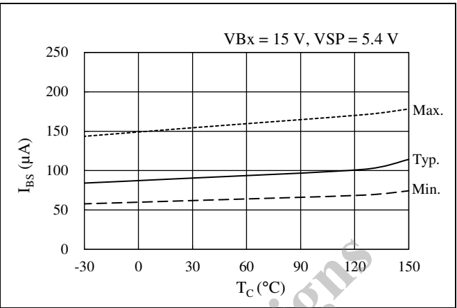
Figure 13-4. Logic Supply Current in 1-phase Operation ( V_{SP} = 5.4 V ), I_{BS} vs. T_C
